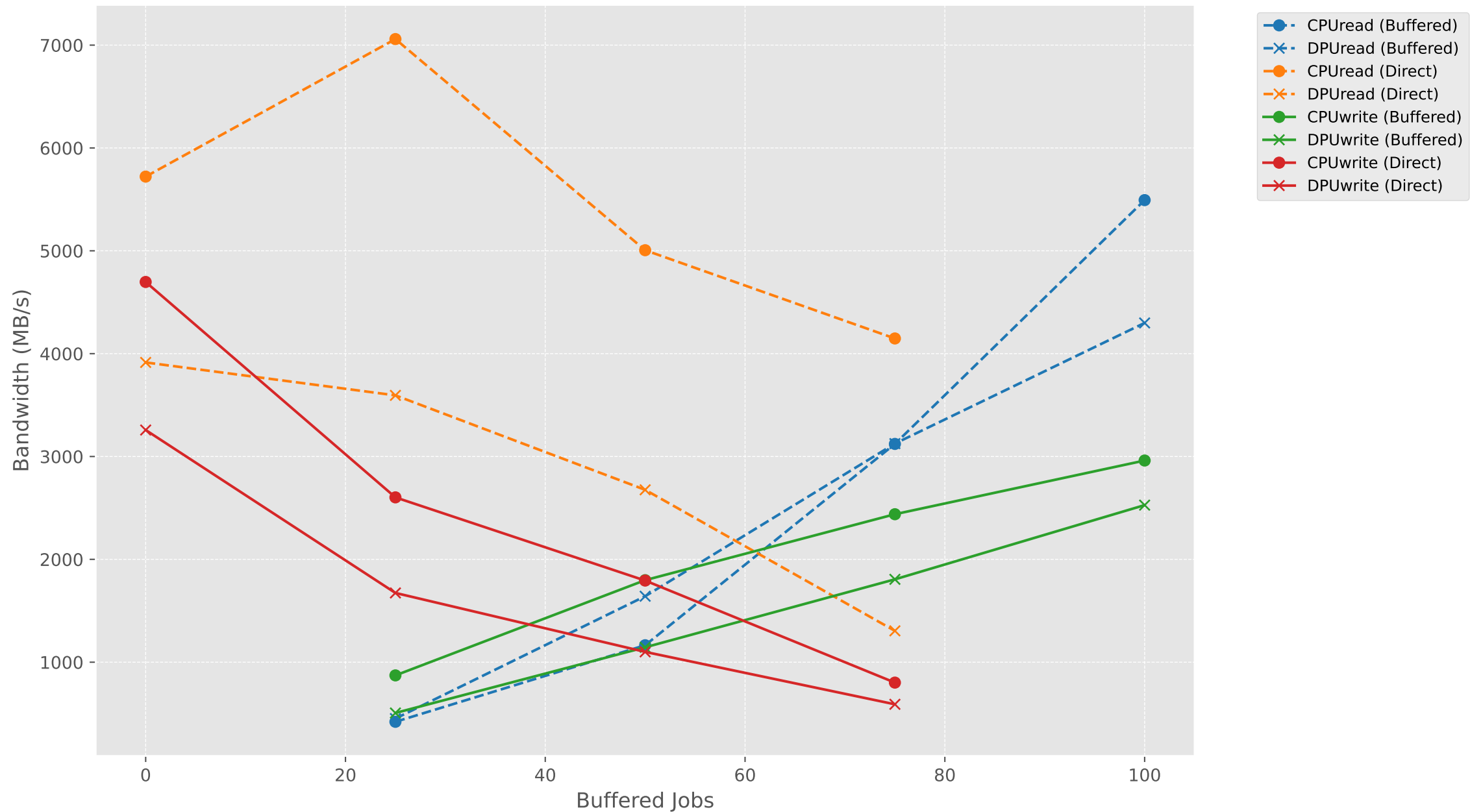
Bandwidth vs Buffered Jobs (mixed) - SEQ (CPU vs DPU)
